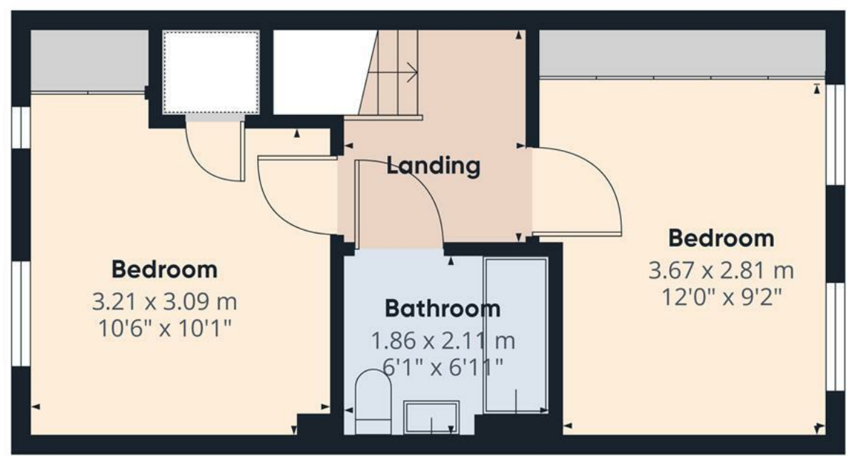
Floor 1
